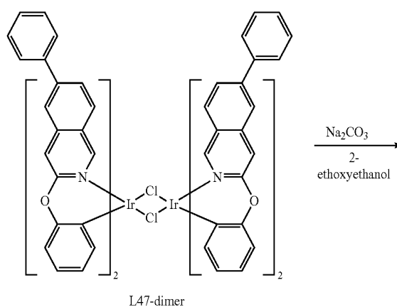
L47-dimer
