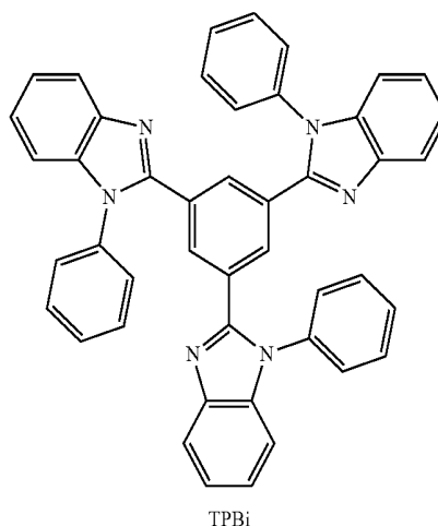
TPBi
